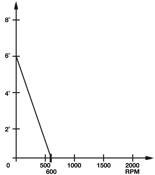
EXAMPLE SPEED TIMING CURVE – ENGINE DEGREES DEGS. RETARD
